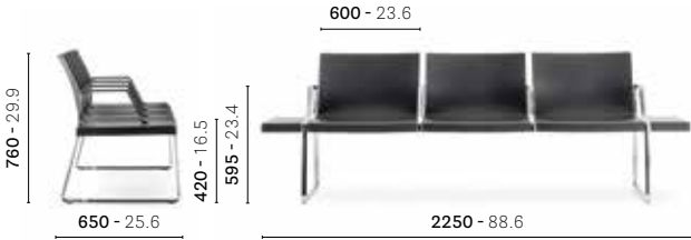
P02013/CL1, P02014/CL1, P02016/CL1, P02019/CL1 Bench multiple seater, polypropylene shell, die-cast aluminium frame with armrests, available in 3, 4, 6 and 9 seats
